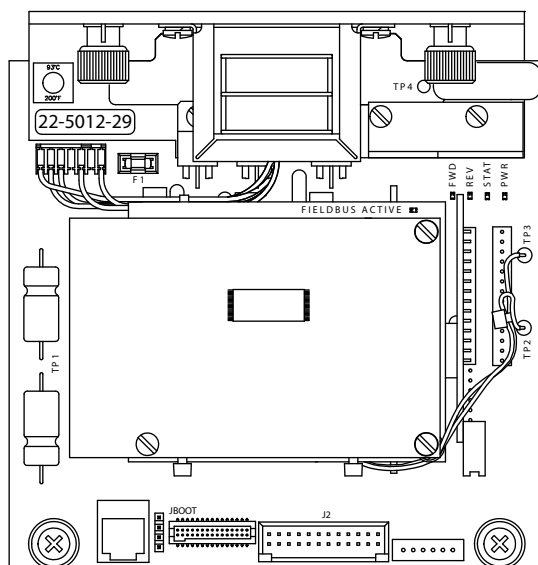
DCM-2 W/ FOUNDATION FIELDBUS
